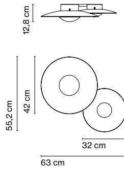
Accessory C2 32/42
